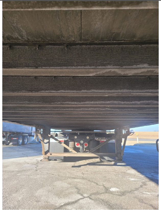
Cross members
